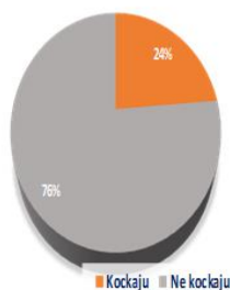
Grafikon 2. Učestalost kockanja ženskih ispitanika izraženo u procentima. Graph 2. Frequency of gambling among female respondents expressed in percentage.
