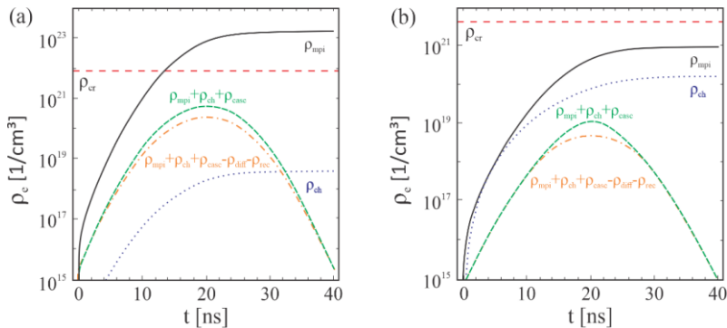
Figure 1. Evolution of the free-electron density across various gain and loss mechanisms at specific wavelengths: (a) 500 nm and (b) 1000 nm.
