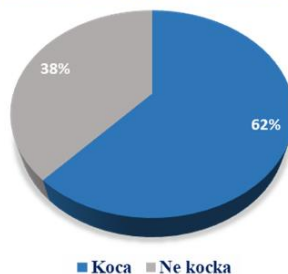
Grafikon 1. Učestalost kockanja muških ispitanika izraženo u procentima. Graph 1. Gambling frequency of male respondents expressed in percentage.
